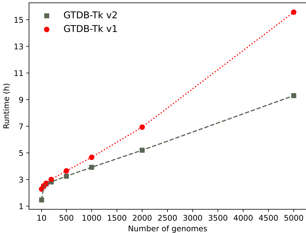
Fig.2: GTDB-Tk runtime with 32CPUs
