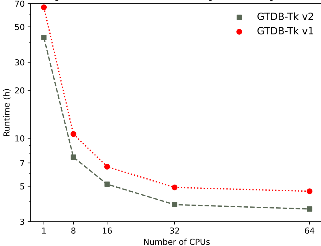
Fig.1: GTDB-Tk runtime for 1000 genomes (log scale)
